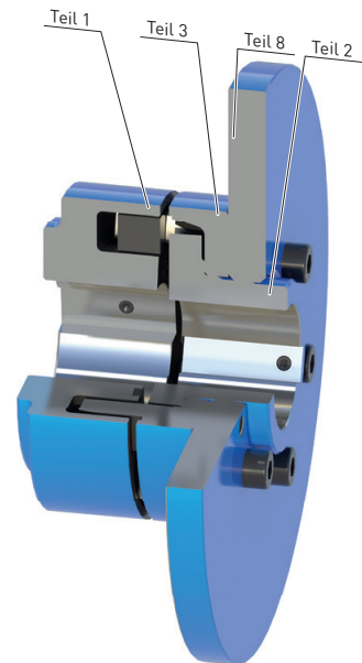
Bauart ABD
