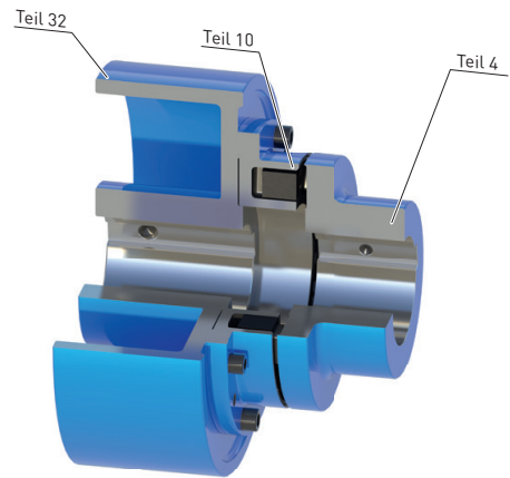
Bauart O
