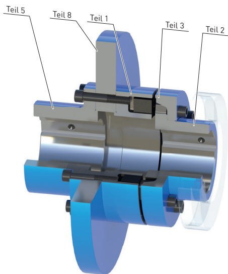
Bauart DBDR
