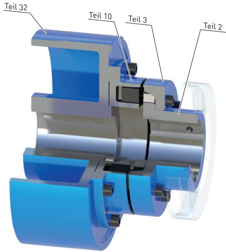
Bauart P
