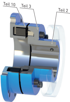
Bauart D
